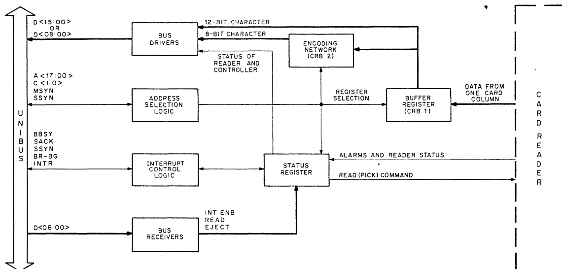
Figure 2-1 CR11 Controller – Simplified Block Diagram
