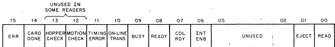
Figure 4-1 Status Register Bit Assignments
