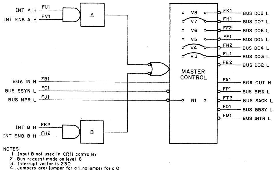
Figure 5-3 Interrupt Control Logic – Simplified Diagram
