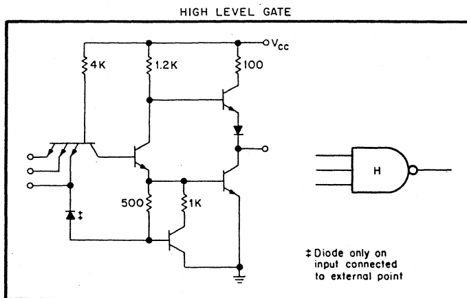
Figure D-3 Circuit Schematic
